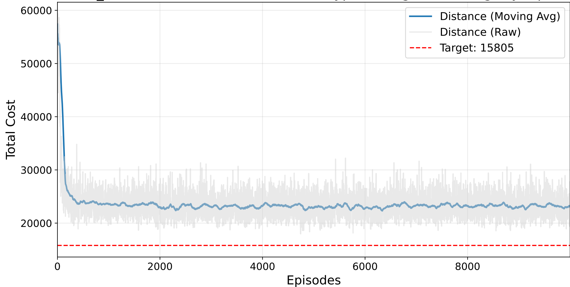
Final NO_BAYESIAN Masked AutoRL-SOP (HyperTuningSK) Training - ry48p.1.sop
